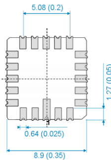
MS9000 bottom view
