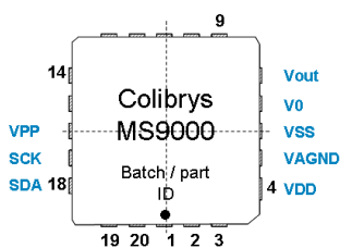
MS9000 top view
